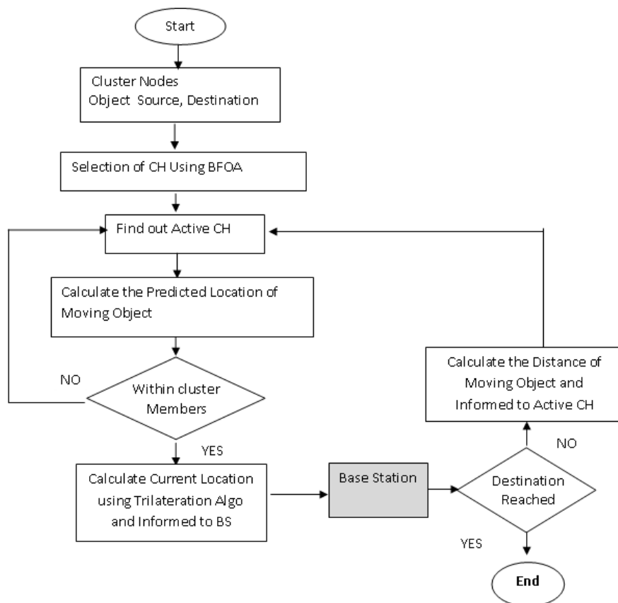
Figure 2: Flowchart of proposed algorithm
